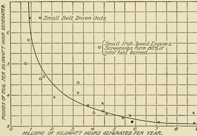
Fig. 163. Curve Showing Relation of Coal Consumption to Quantity of Energy Generated
